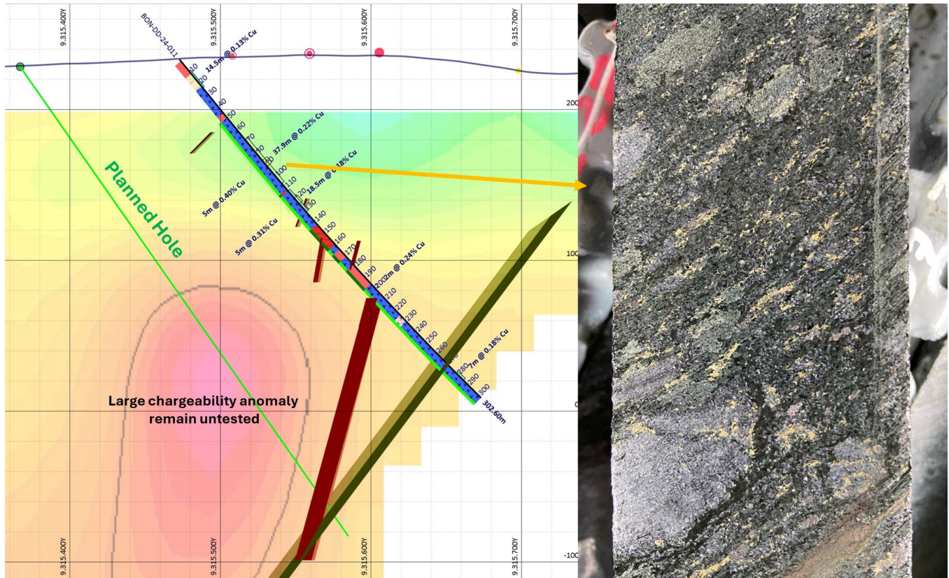
Figure 7 – Nelore Prospect – Section 658300mE and core photo from drill hole BON-DD-24-011; 86m down-hole: disseminated to stringer sulphides – chalcopryite (brassy yellow) > pyrrhotite (brown-bronze colour) > pyrite (distinguished by hardness test) – returned 5.0m at 0.40% Cu and 0.11 ppm Au
